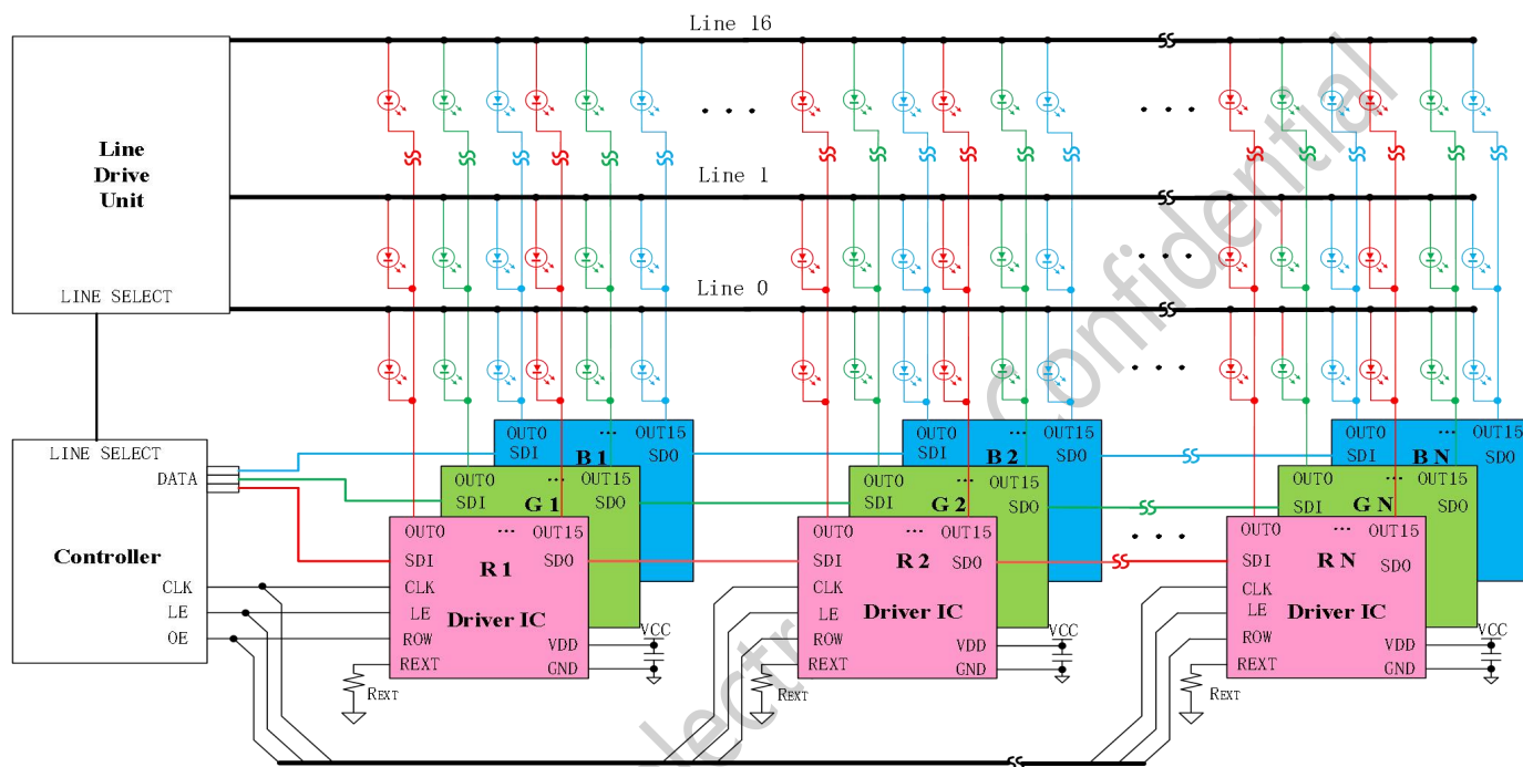
LED 显示屏 16 扫应用框图
