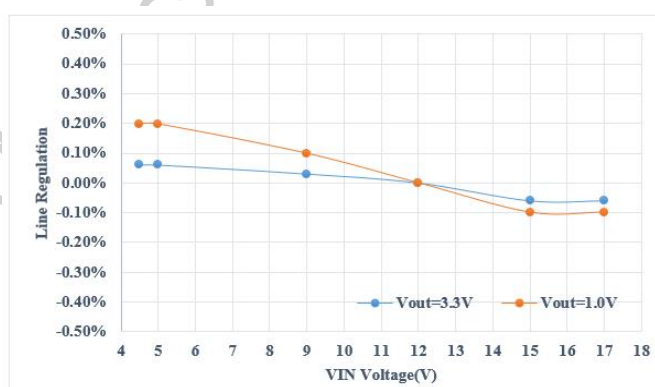
Figure4 Line Regulation Iout=1A
