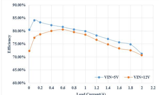
Figure2 1.0V Output Efficiency
