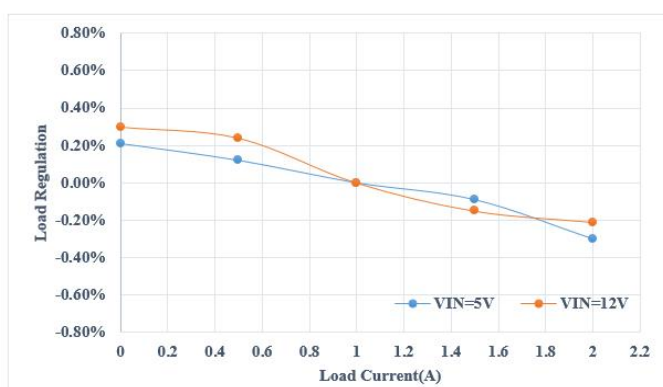
Figure3 Load Regulation
