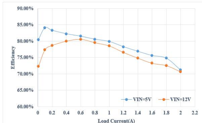
Figure2 1.0V Output Efficiency
