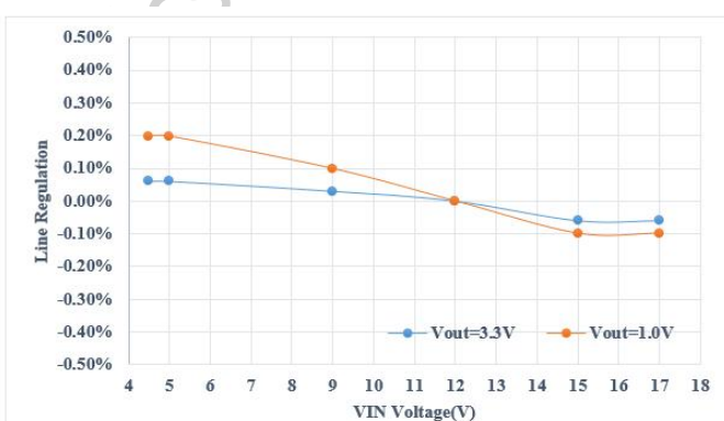
Figure4 Line Regulation Iout=1A
