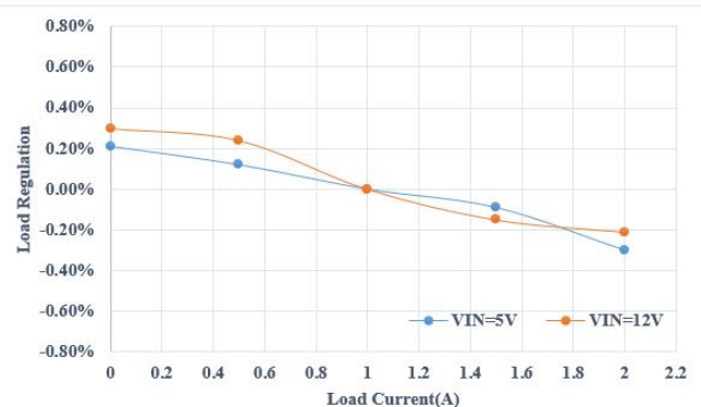
Figure3 Load Regulation
