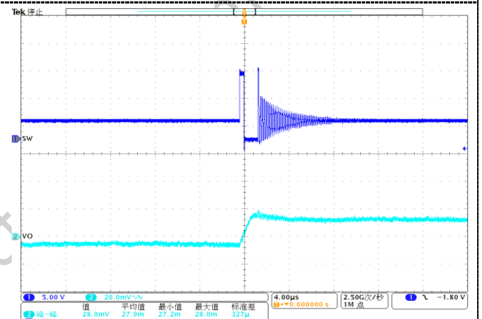
Iout=0 A Figure10 DCM Mode
