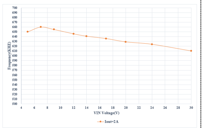
Figure6 Switch Frequency vs VIN
