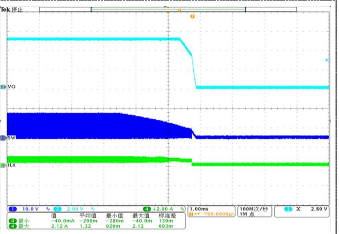
Iout=2A Figure12 EN ShutDown with Load
