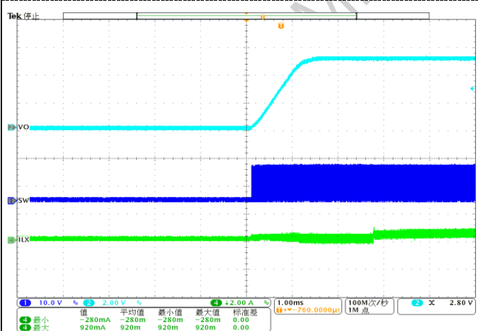
Iout=2A Figure11 EN StartUp with Load
