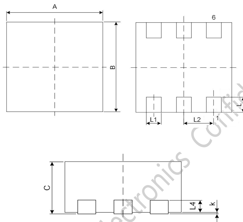
DFN1.6×1.6-6
