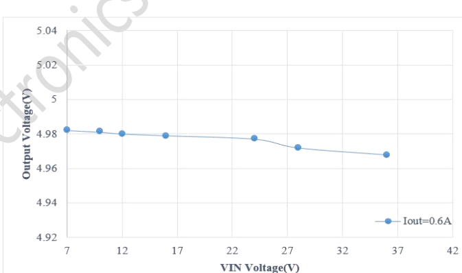
Figure4 Line Regulation I_{out}=0.6\text{A}
