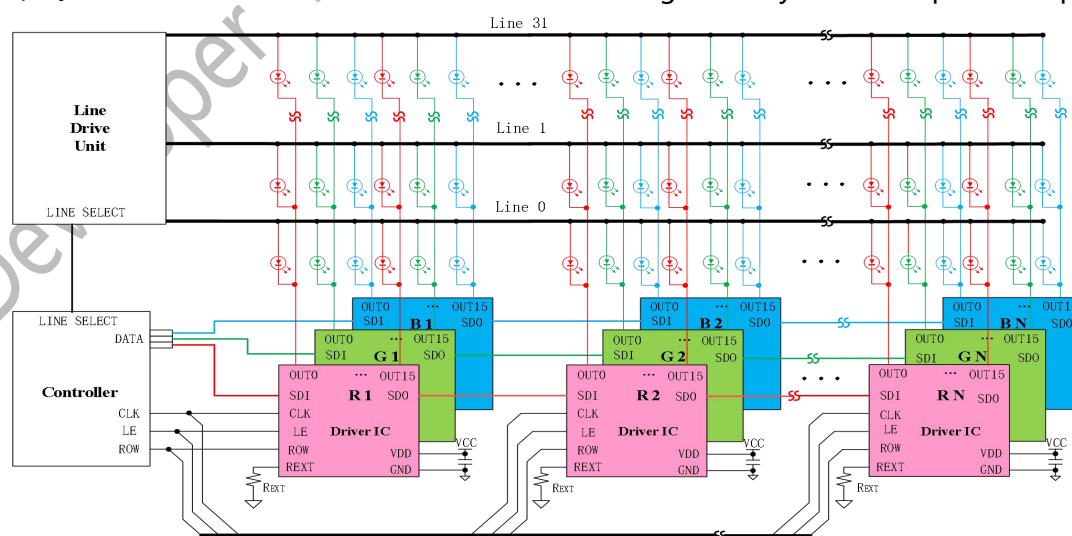
DP3153 Typical Application Schematic
