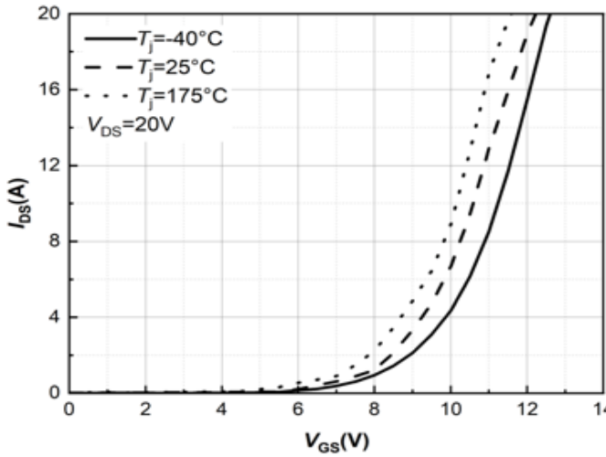
Fig 7: Transfer Characteristics
