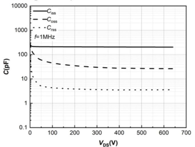
Fig 12: Capacitance Characteristics
